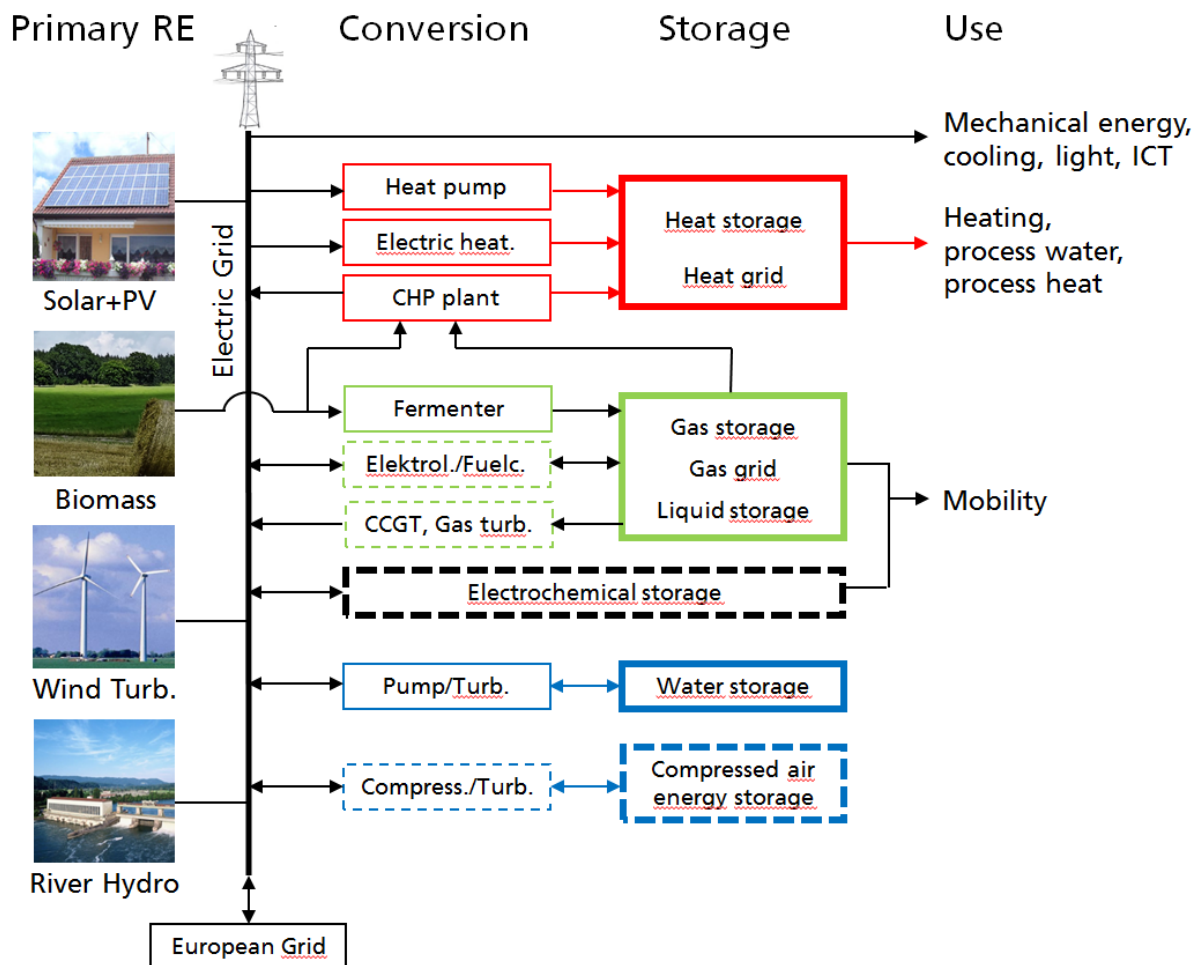
Figure 60: Simplified scheme of a Renewable Energy System with the most important grid-related components of the categories production, conversion, storage and consumption.
