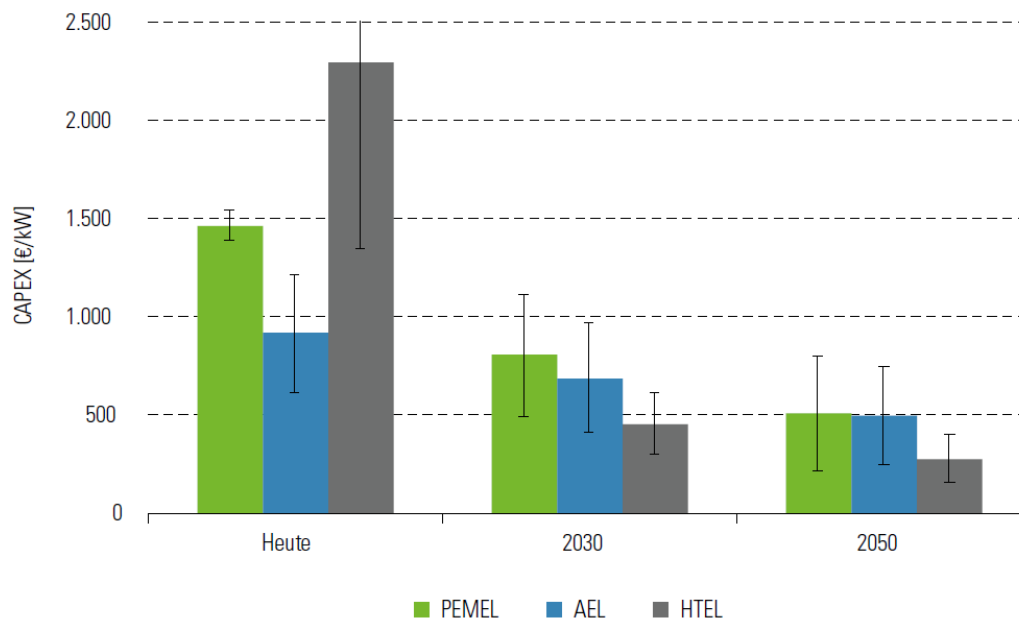
Figure 57: Specific investment costs for different electrolyzer technologies (PEMEL: Membrane electrolysis, AEL: Alkaline electrolysis, HTEL: High-temperature electrolysis, [NOW])
