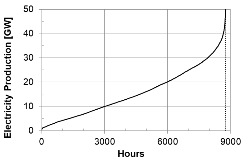
Figure 54: Fictitious annual electricity production (8760 hours) for 200 GW p PV and 200 GW p wind, extrapolated on the basis of installation and yield data for 2017
