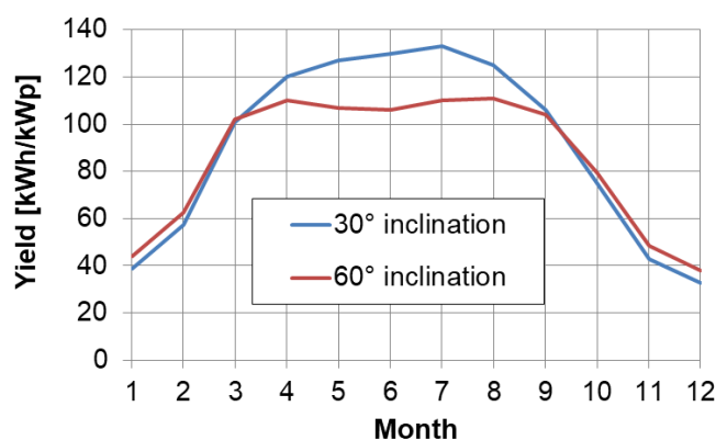
Figure 51: Calculation example for the specific monthly yield of a PV system at Freiburg for south-oriented modules with 30° inclination (maximum annual yield) and 60° inclination.
