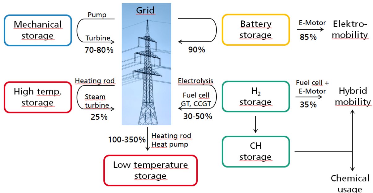
Figure 58: Technologies for energy storage and converters with today's achievable efficiencies at the end of the converter chain, without combined heat and power
