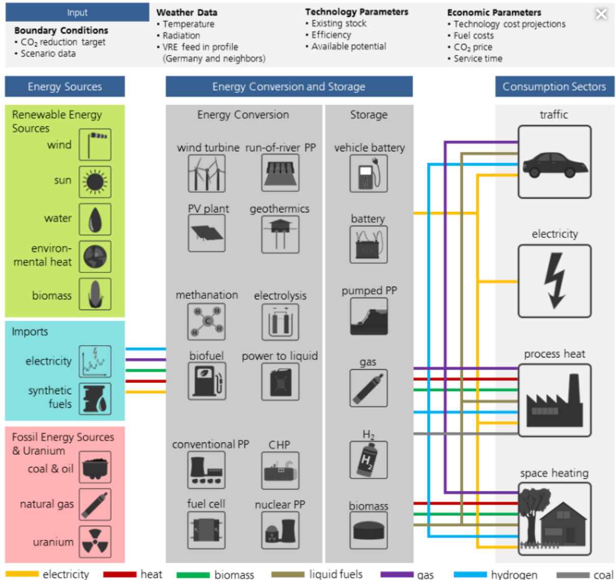
Figure 46: Schematic representation of the REMod model [ISE12]
