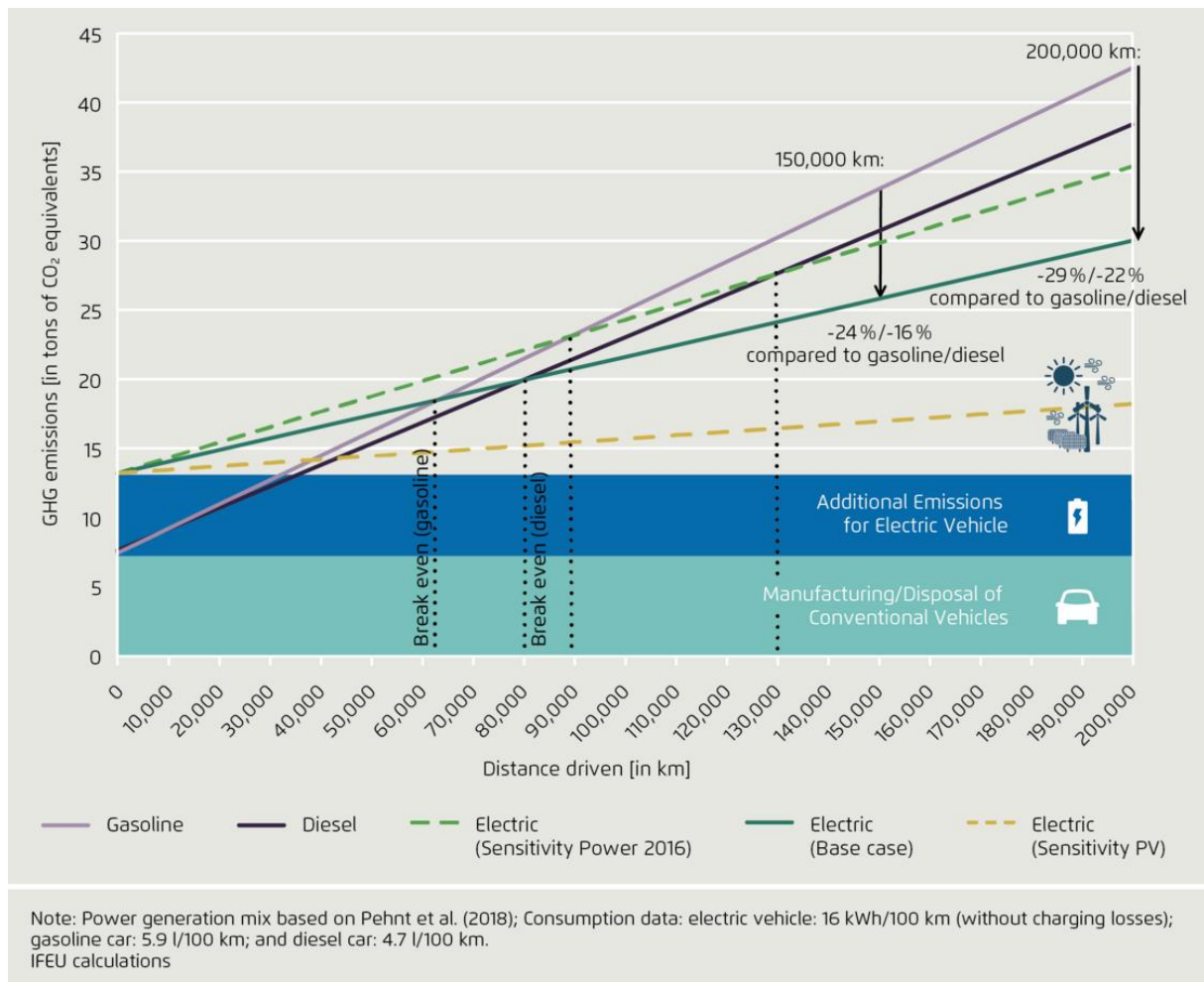
Figure 53: Greenhouse gas emissions of today's compact-class vehicles as a function of mileage [AGORA2]
