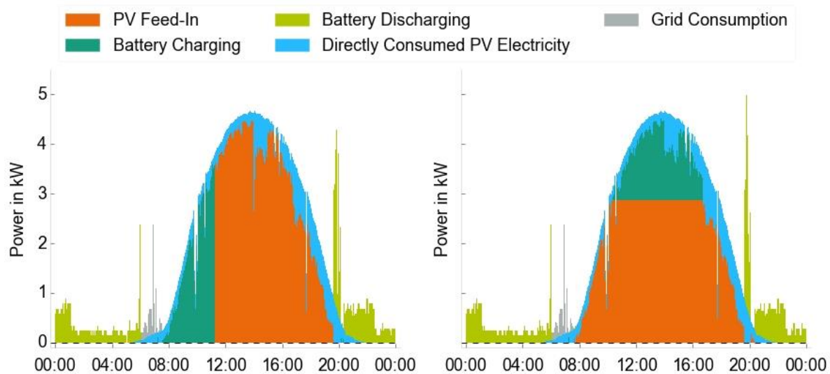
Figure 56: Comparison of the conventional and grid-optimized system operation [ISE7]
